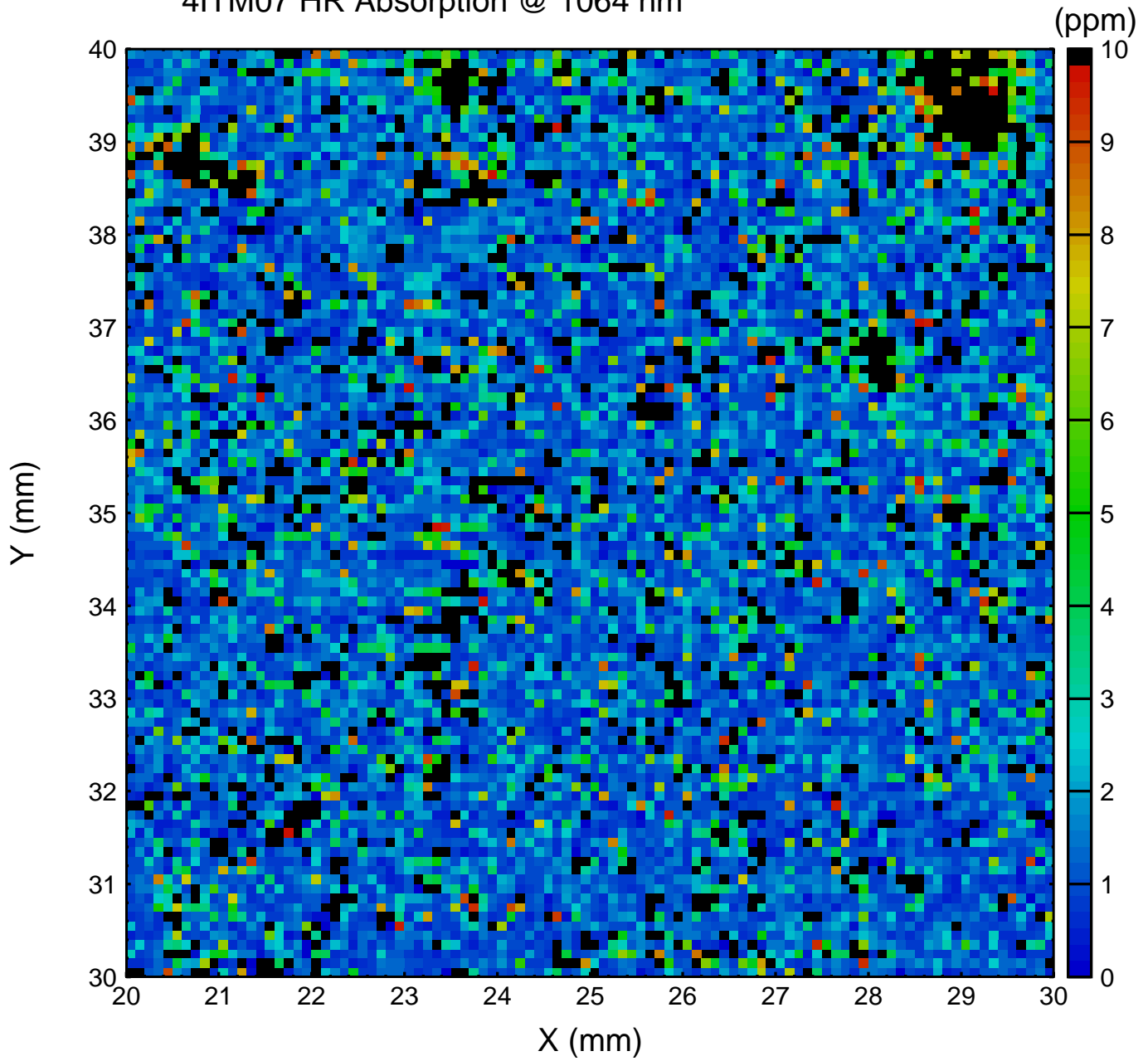
4ITM07 HR Absorption @ 1064 nm
