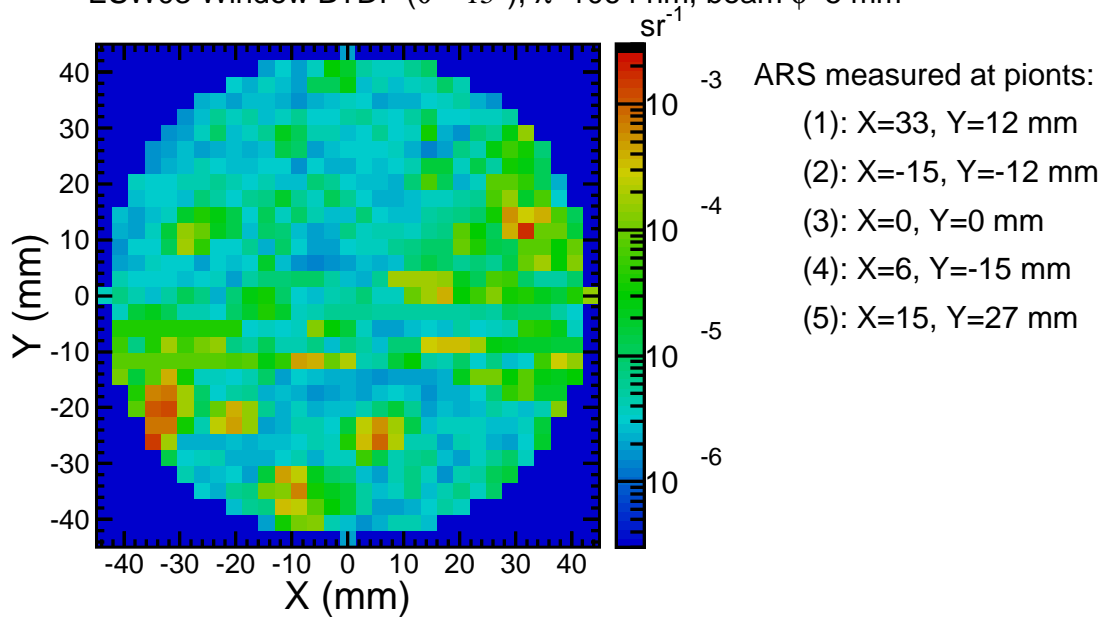
ESW03 Window BTDF ( \theta = 15^\circ ), \lambda=1064 nm, beam \phi=5 mm
