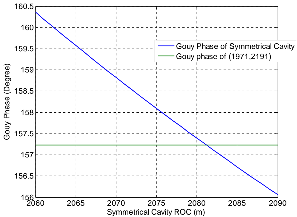
Fig. 2: Gouy phase of the symmetrical cavity with a reference line for the current (1971,2191) m cavity design
