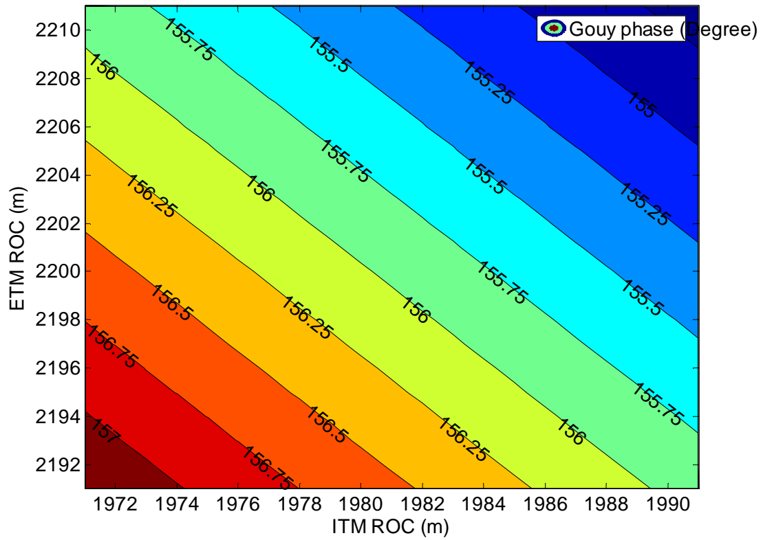
Fig. 3: Gouy phase of the Unsymmetrical cavity for the range of ITM/ETM ROC
