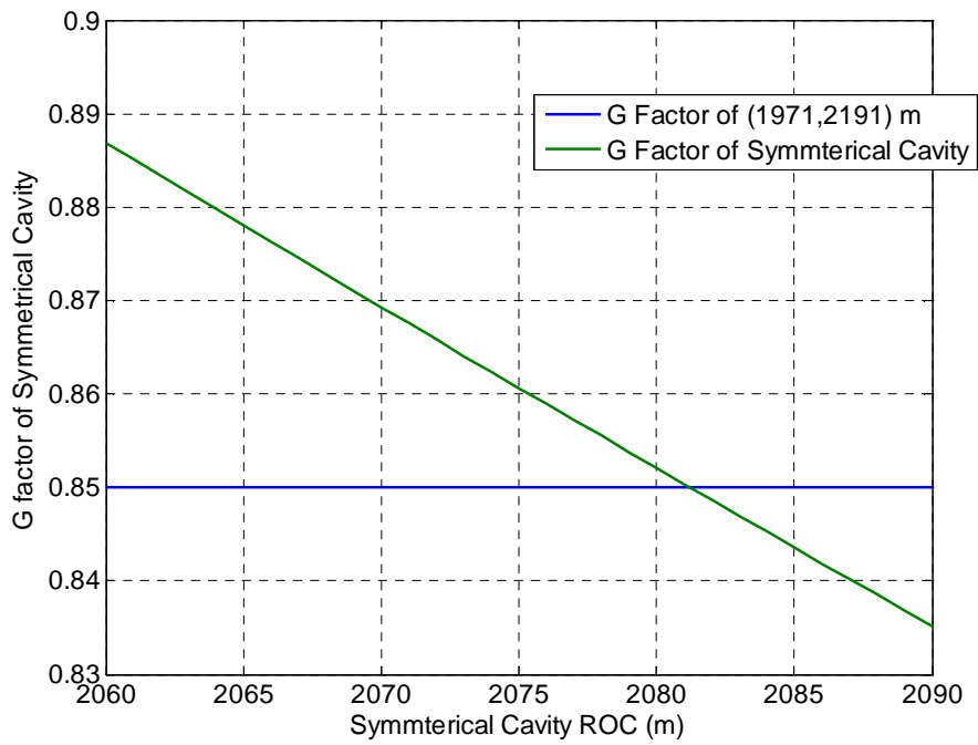
Fig. 1: G factor of the symmetrical cavity with a reference line for the current (1971,2191) m cavity design
