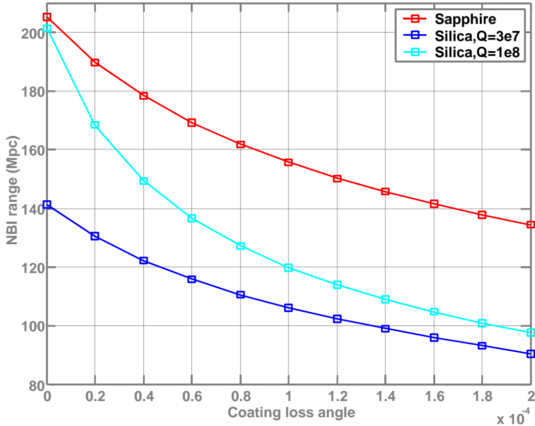
Figure 3. Neutron star binary inspiral range for a single interferometer of the indicated test mass material, as a function of the optical coating mechanical loss. Calculations are made with Bench 1.13, with coating thermal noise approximated by equation 23 of Harry et al 6 .
