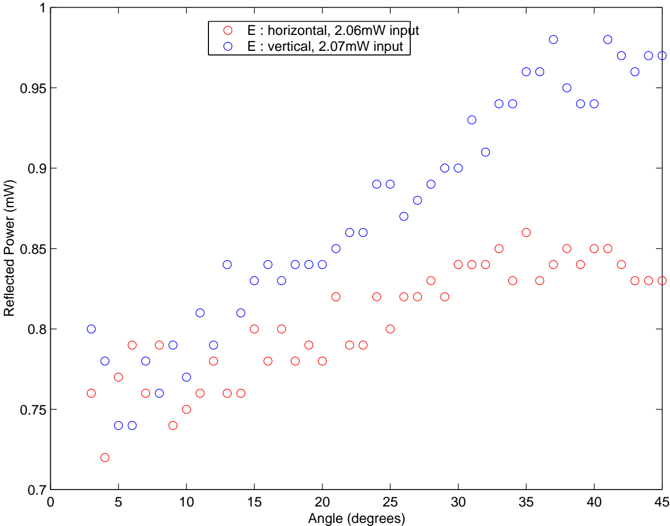
Reflectivity measurement for RM03/04 Witness optic (HR)
