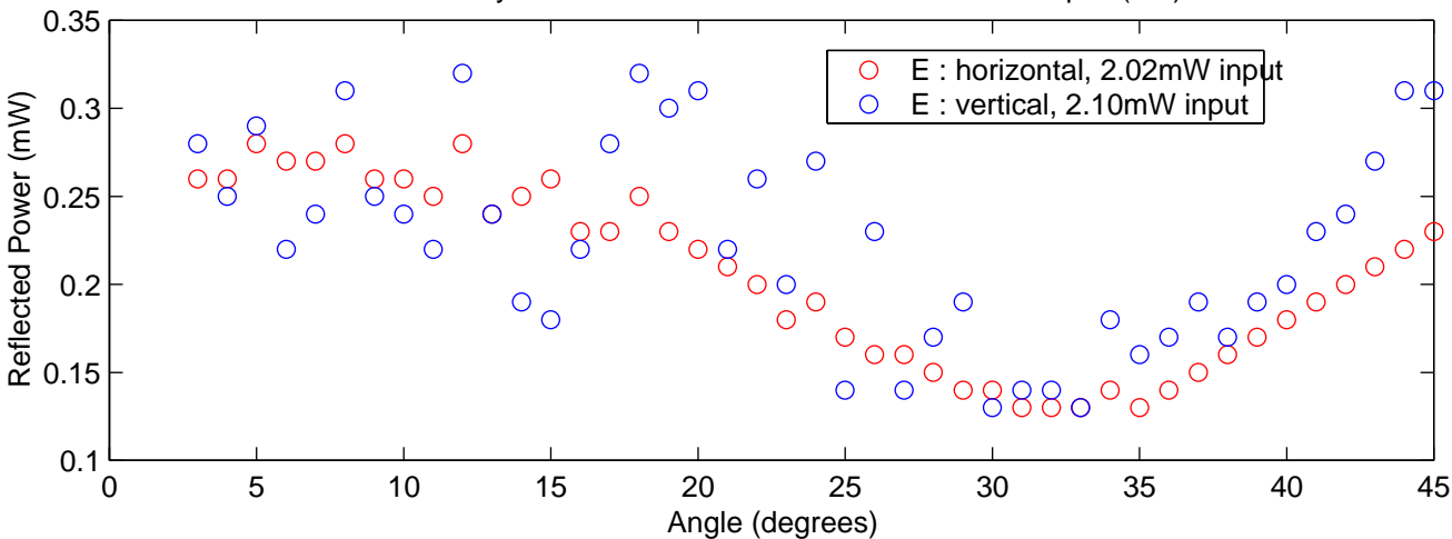
Reflectivity measurement for SPETM05/07 Witness optic (HR)
