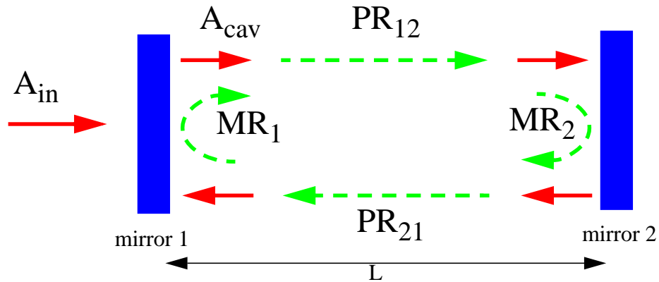
Figure 4: FP cavity schematics
