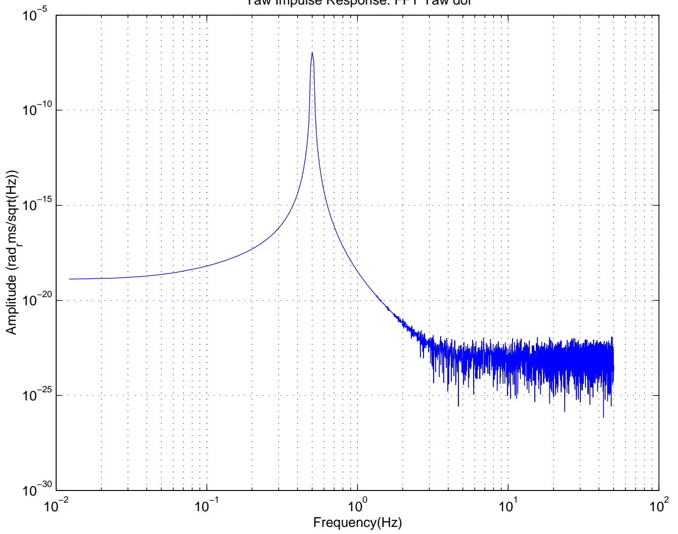
Yaw Impulse Response: FFT Yaw dof
