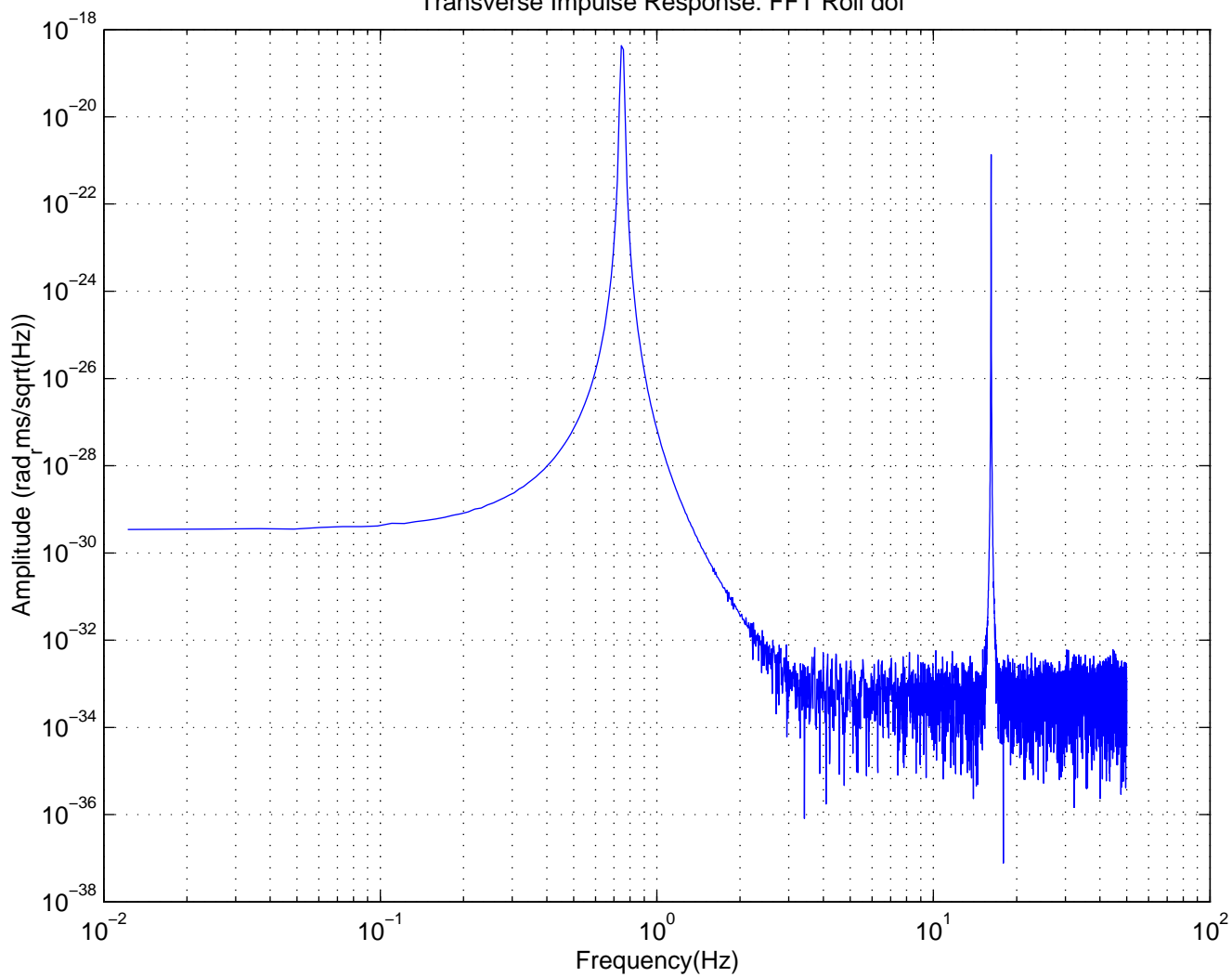
Transverse Impulse Response: FFT Roll dof
