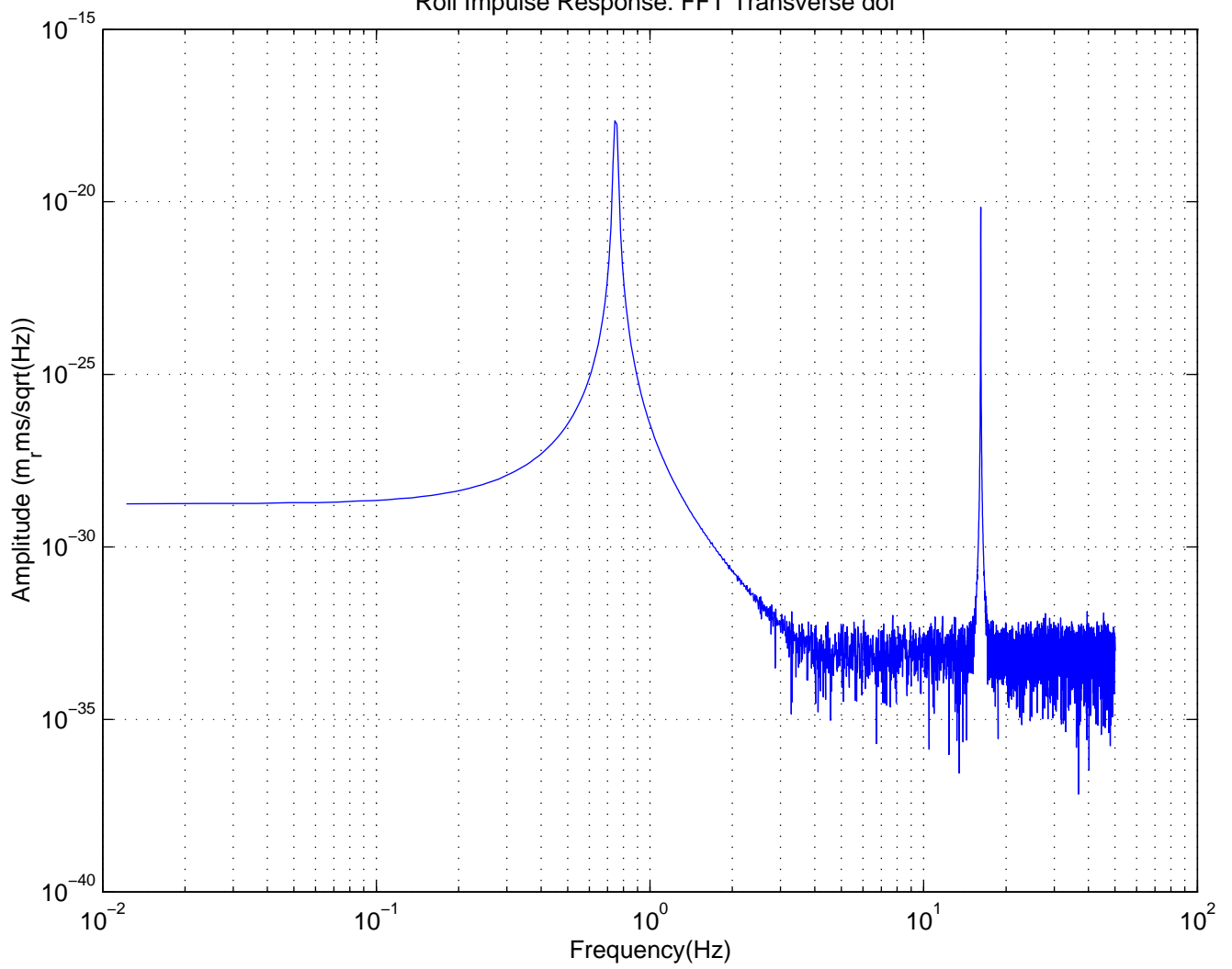
Roll Impulse Response: FFT Transverse dof
