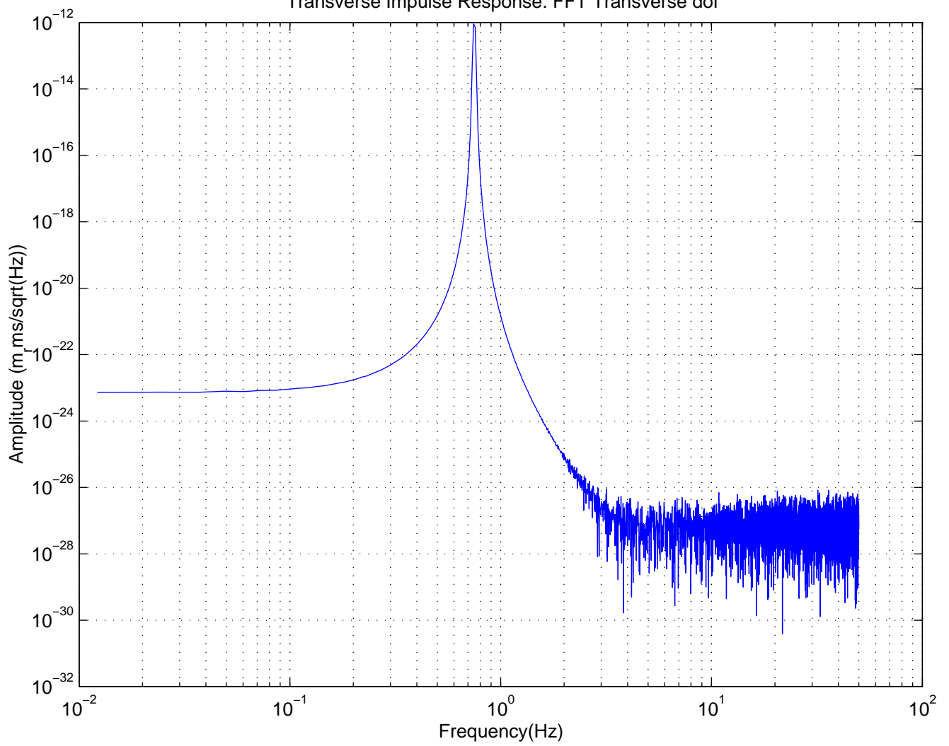
Transverse Impulse Response: FFT Transverse dof
