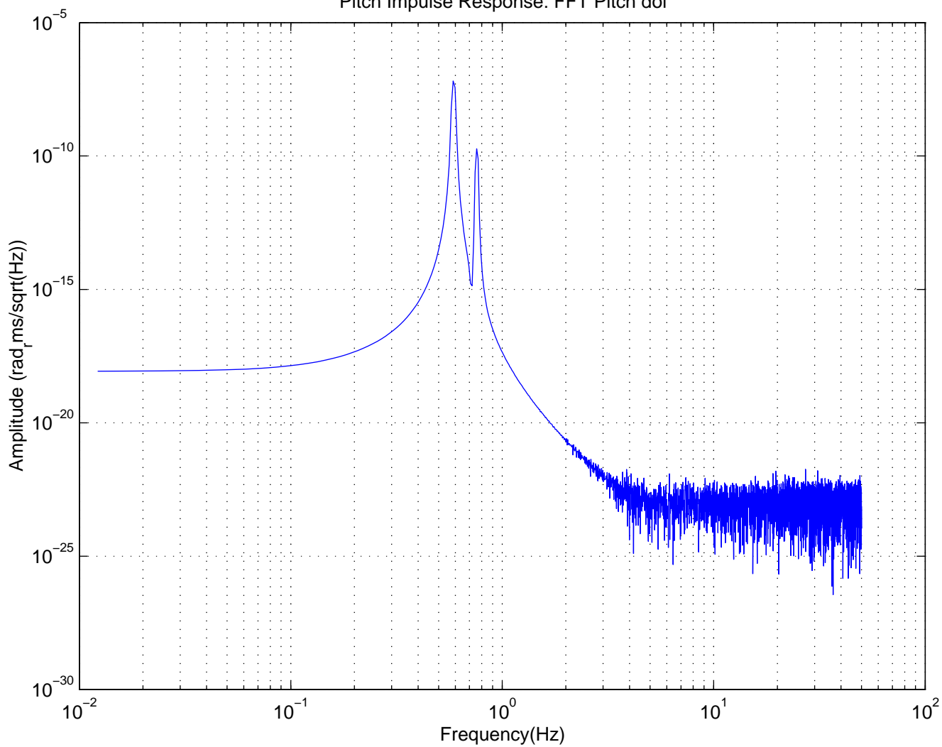
Pitch Impulse Response: FFT Pitch dof
