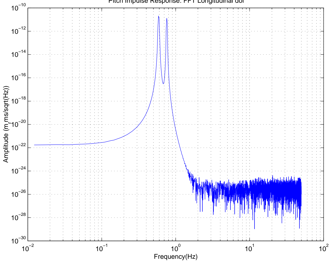
Pitch Impulse Response: FFT Longitudinal dof
