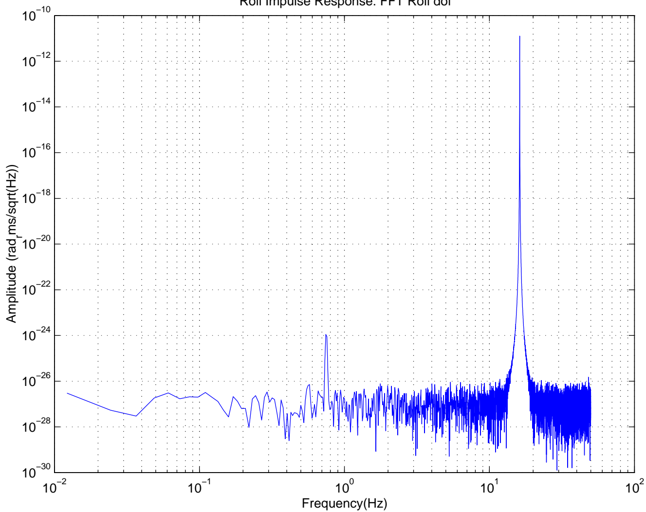
Roll Impulse Response: FFT Roll dof
