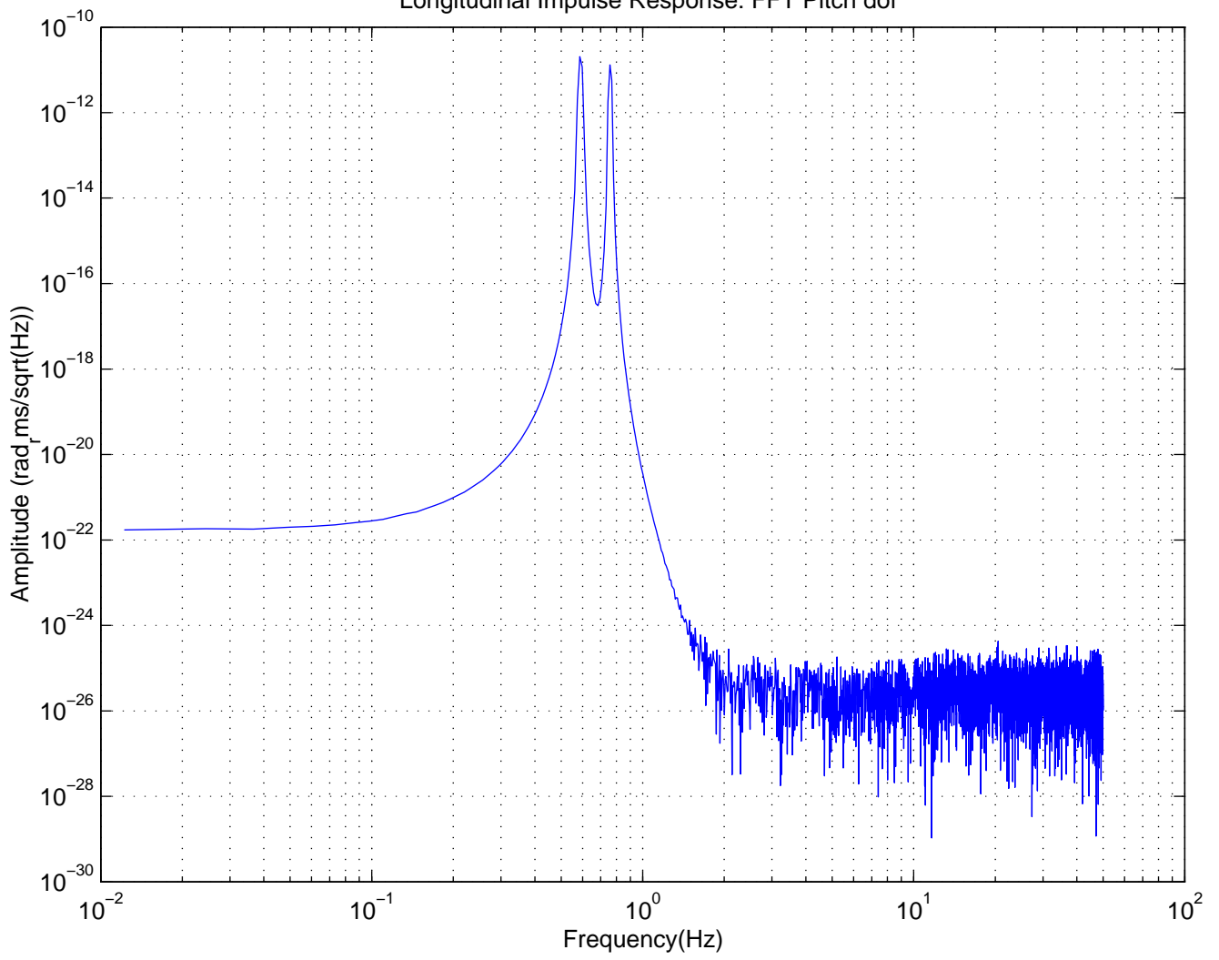
Longitudinal Impulse Response: FFT Pitch dof
