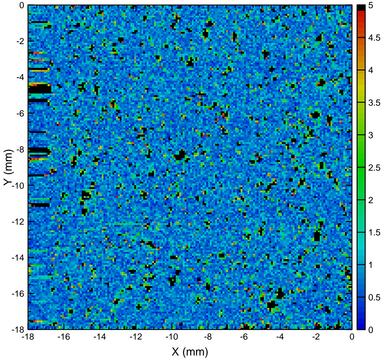
4ITM07 HR Absorption @ 1064 nm (ppm)
