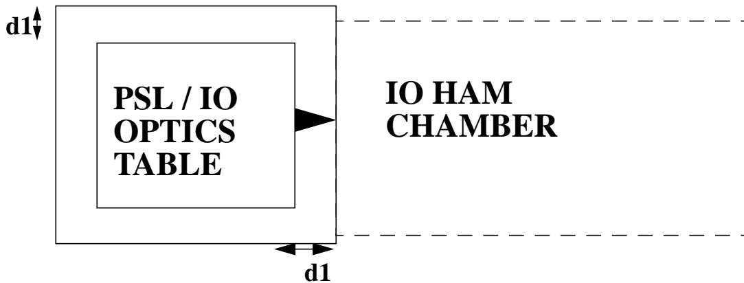
Figure 3: Stay clear dimensions
