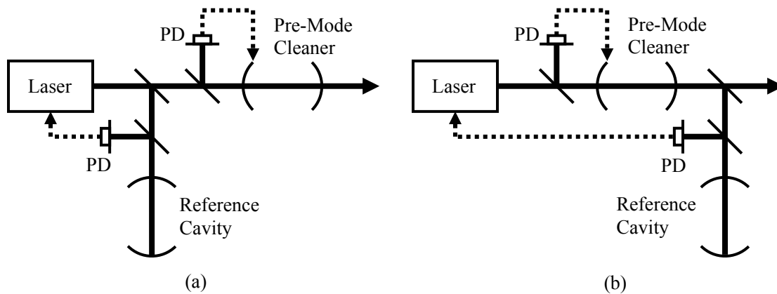
Fig. 1 Configurations of the pre-stabilized Laser with the light picked off for the reference cavity (a) before the pre-mode cleaner and (b) after the pre-mode cleaner.
