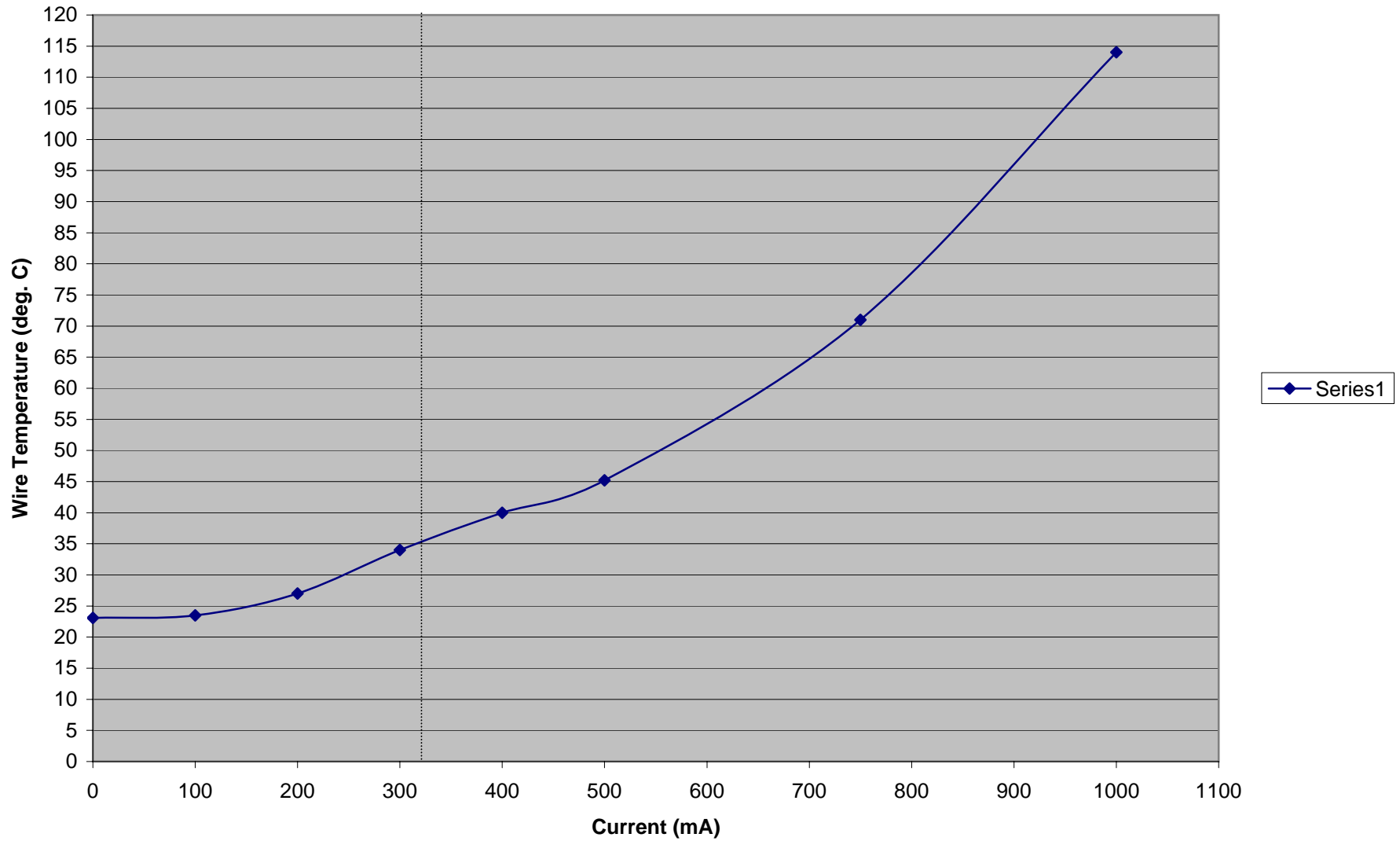
Wire Temperature vs. Current
