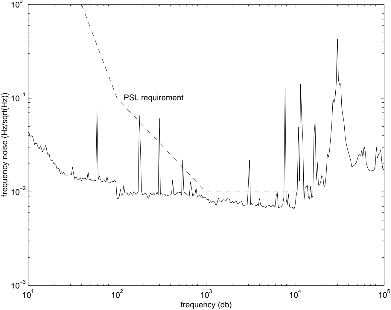
FSS In-loop Frequency Noise 10/23/01
