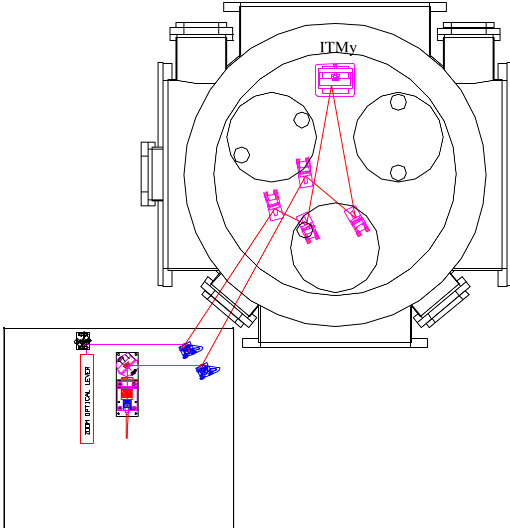
Figure 8: Optical lever, ITMy
