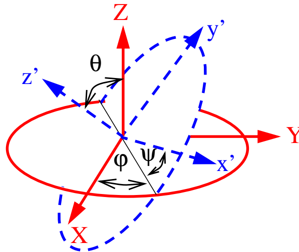
Figure 13: Euler angles
