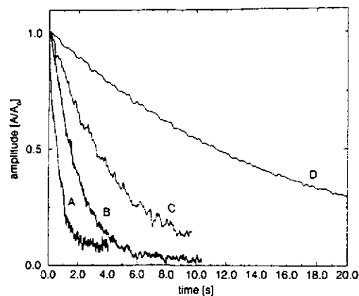
Fig. 2. Averaged decay traces (normalized) for suspensions produced with the bonding methods described in the text. See Table 1 for experimental data of the traces.
