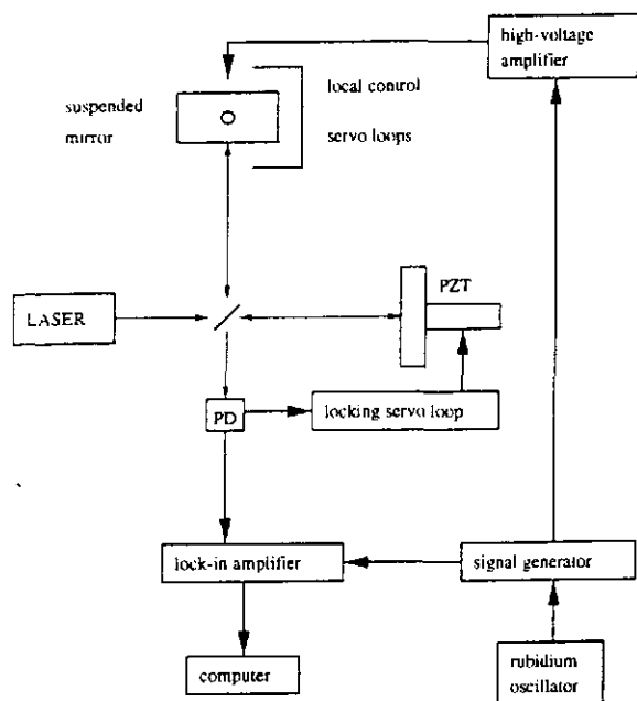
Fig. 1. Schematic diagram of the experimental arrangement used to measure the internal mechanical quality factor of substrates monolithically suspended on single fibres.
