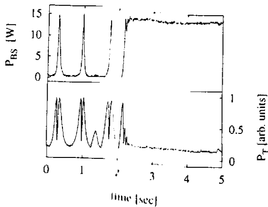
Fig. 4. The measured transmitted and internal powers, P_T and P_{BS} , with the 7% PR-mirror during the second step of acquiring lock. The fluctuating MI-phase is locked to the dark fringe at t = 2.1 s.
