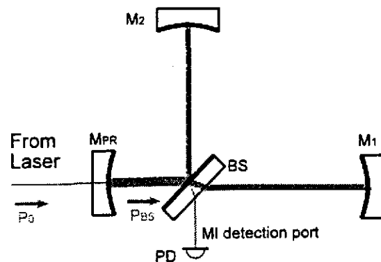
Fig. 1. Michelson interferometer (BS, M_1 , M_2 ), with power-recycling mirror M_{PR} added.
