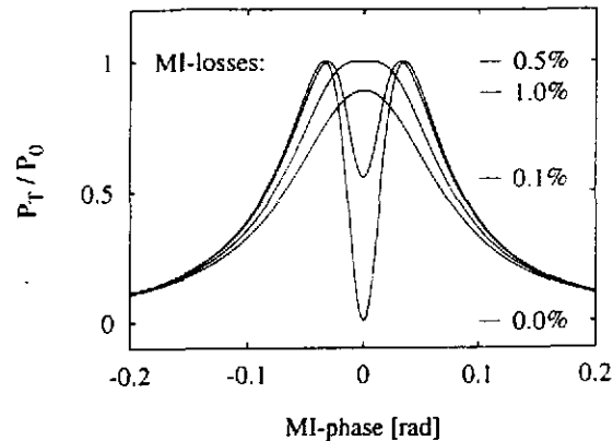
Fig. 2. Calculated light power P_T at the detection port of a power recycled Michelson, as a function of the MI-phase. (The PR-cavity is assumed to be kept on resonance.) Assumptions are \tau_{PR}^2 = 0.5\% and different values of MI-losses A due to an anti-symmetric end-mirror deformation.
