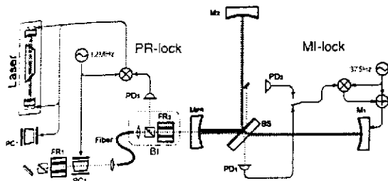
Fig. 3. Experimental set-up.
