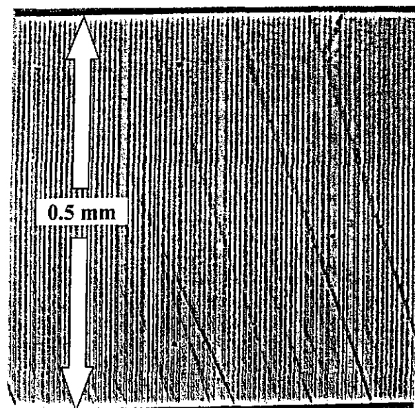
Fig. 1. Etched y face of 0.5-mm-thick periodically poled LiNbO 3 showing 6.5- \mu\text{m} period domains. The domain duty cycle is approximately 35%. The diagonal features are polishing scratches.
