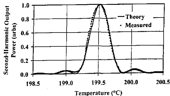
Fig. 2. 532-nm output power [in arbitrary units (arbs)] versus temperature for Nd:YAG SHG. The dots are experimental data, and the solid curve is the theoretical plane-wave curve for a 53-mm sample, shifted to the same peak phase-matching temperature. The good agreement between data and theory indicates the sample phase matches over the full 53-mm length.
