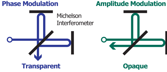
Figure 2. The Schnupp asymmetry designs for both modulations. The phase modulation mod-1 transmits the MI completely, so the MI acts as a simple steering mirror, meanwhile, the amplitude modulation mod-2 is reflected by the MI completely, so the MI acts as an ideal reflecting mirror.
