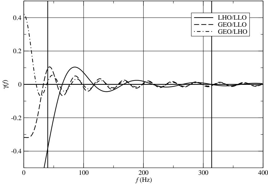
Figure 1. The overlap reduction function \gamma(f) for combinations of the LIGO Livingston Observatory (LLO) and LIGO Hanford Observatory (LHO) with each other and with the GEO600 site. (GEO600 was also operational during S1, but has not been included in this analysis because it was considerably less sensitive than the LIGO detectors.) Note that the overlap reduction function for correlations between the two detectors at LHO (H1 and H2) is identically equal to unity. The solid lines (at f = 40 Hz and 314 Hz) show the range of frequencies used in our analysis.
