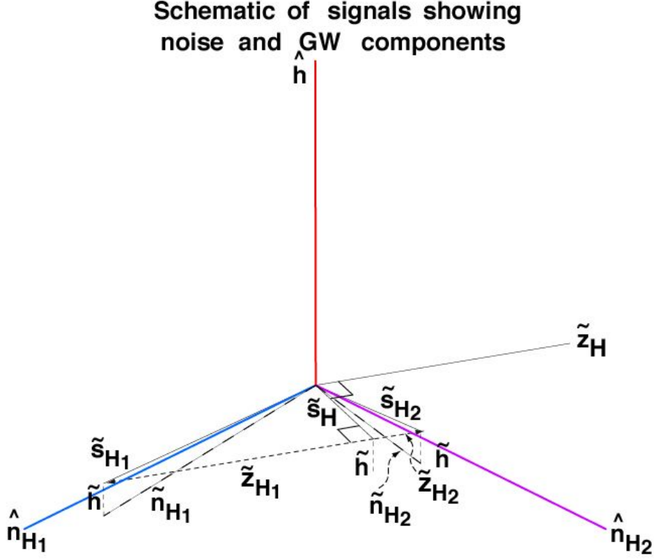
FIG. 4: Schematic showing how the H1 and H2 signals may be represented in a 3-dimensional space of noise components for the two detectors and the common gravitational wave strain: \{\hat{n}_{H1}, \hat{n}_{H2}, \hat{h}\} . The signals \tilde{s}_{H1}(f) and \tilde{s}_{H2}(f) are not, in general, orthogonal if the coherence between the noise, \tilde{n}_{H1}(f) and \tilde{n}_{H2}(f) , is non-zero. \tilde{s}_H(f) is the minimum variance estimate of \tilde{h}(f) derived from \tilde{s}_{H1}(f) and \tilde{s}_{H2}(f) . Using \tilde{s}_H(f) as the best estimate of \tilde{h}(f) , this signal can be subtracted from \tilde{s}_{H1}(f) and \tilde{s}_{H2}(f) to produce the vectors \tilde{z}_{H1}(f) , \tilde{z}_{H2}(f) that lie in the \hat{n}_{H1} - \hat{n}_{H2} plane. These vectors give rise to the covariance matrix \|\tilde{\mathbf{C}}_z(f)\| . \tilde{z}_{H1}(f) and \tilde{z}_{H2}(f) are colinear and thus one of the eigenvectors of \|\tilde{\mathbf{C}}_z(f)\| will be zero. The other corresponds to the dual of \tilde{s}_H(f) , denoted \tilde{z}_H(f) , which is orthogonal to \tilde{s}_H(f) , as shown in the figure. Note that it is necessary to first subtract the contribution of \tilde{h}(f) from the signals before forming the covariance matrix.
