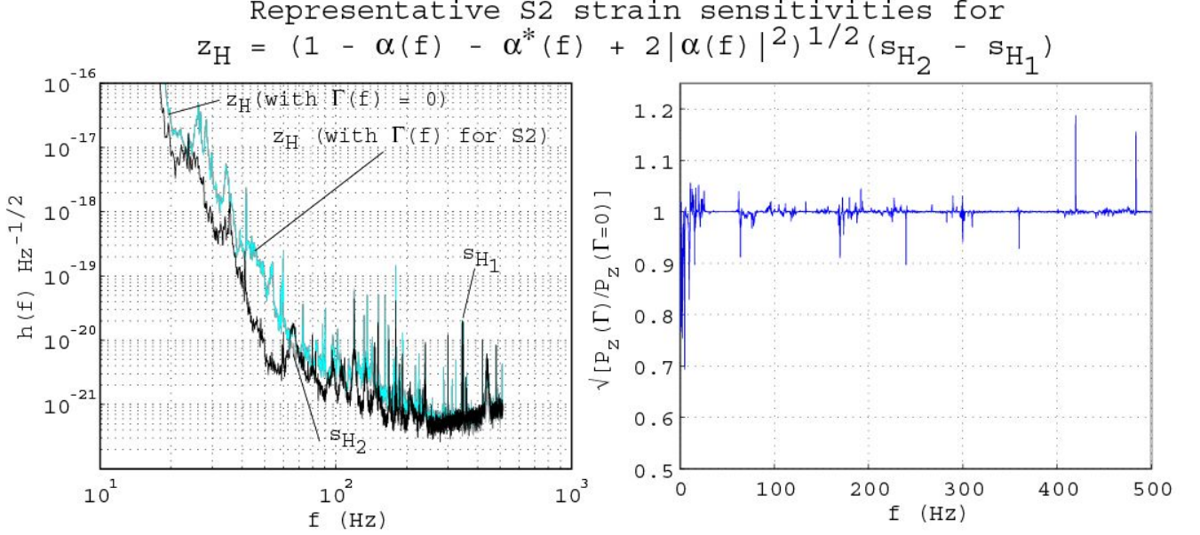
FIG. 3: Same as Fig. 1, but for the null signal \tilde{z}_H(f) instead of the optimal estimate \tilde{s}_H(f) . Strain spectral densities (i.e., absolute value) of \tilde{z}_H(f) (colored), \tilde{s}_{H_1}(f) (black), and \tilde{s}_{H_2}(f) (grey), representative of the S2 data. Left Panel: overlay of the individual amplitude spectral densities with that of the strain spectral density |\tilde{z}_H(f)| is calculated with the S2 run-averaged coherence, \Gamma_{H_1H_2}(f) . On this scale, the left hand panel shows no discernible difference between the spectra for \Gamma_{H_1H_2}(f) , and with \Gamma_{H_1H_2} = 0 , suggesting that even the level of coherence seen during the S2 run might be sufficiently low to allow one to simply combine the L1-H1 and L2-H2 cross-correlation measurements under the assumption of zero cross-correlated noise. Referring to the discussion in Appendix B, the optimality of the estimate \tilde{z}_H(f) is visible here because it is always less than the larger of \tilde{s}_{H_1}(f) or \tilde{s}_{H_2}(f) . Right panel: overlay of individual amplitude spectra with that for |\tilde{z}_H(f)| calculated with \Gamma_{H_1H_2}(f) = 0 (i.e., assuming no coherence). The difference between the two is very small except for the very lowest frequencies and at narrow line features.
