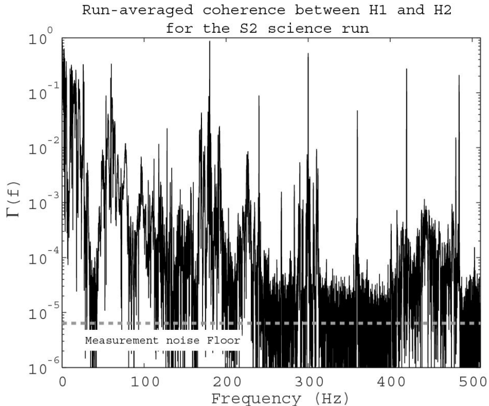
FIG. 2: H1-H2 coherence averaged over the whole S2 data run. Note the substantial broadband coherence below 250 Hz and between 400 and 475 Hz. Low frequency seismic noise and acoustic coupling between the input electro-optics systems are considered to be the prime sources of this cross-correlated noise [6, 7].
