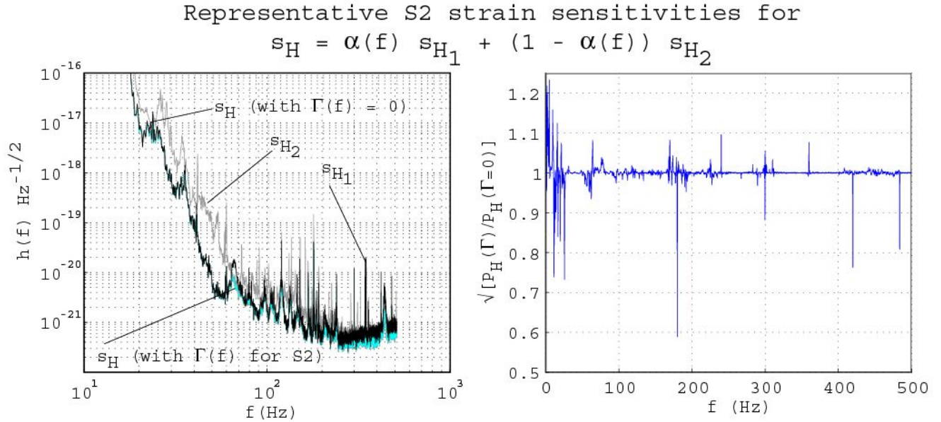
FIG. 1: Strain spectral densities (i.e., absolute value) of \tilde{s}_H(f) (colored), \tilde{s}_{H_1}(f) (black), and \tilde{s}_{H_2}(f) (grey), representative of the S2 data. Left Panel: overlay of the individual spectral densities with that of the strain spectral density |\tilde{s}_H(f)| calculated with the S2 run-averaged coherence, \Gamma_{H_1H_2}(f) , and with \Gamma_{H_1H_2}(f) = 0 . On this scale, the left hand panel shows no discernible difference between the spectra for \Gamma_{H_1H_2}(f) , and with \Gamma_{H_1H_2}(f) = 0 , suggesting that even the level of coherence seen during the S2 run might be sufficiently low to allow one to simply combine the L1-H1 and L2-H2 cross-correlation measurements under the assumption of zero cross-correlated noise. Referring to the discussion in Appendix A, the optimality of the estimate \tilde{s}_H(f) is visible here because it is always less than the smaller of \tilde{s}_{H_1}(f) or \tilde{s}_{H_2}(f) . Right panel: plot of the ratio of amplitude spectra for |\tilde{s}_H(f)| calculated with \Gamma_{H_1H_2}(f) as measured during S2 and \Gamma_{H_1H_2}(f) = 0 (i.e., assuming no coherence). The difference between the two is very small except for the very lowest frequencies and at narrow line features.
