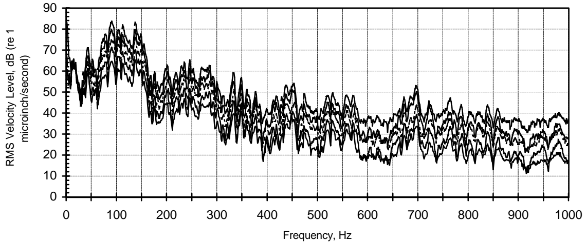
a) Noise induced panel vibration: narrowband (effective bandwidth = 1.875 Hz)
