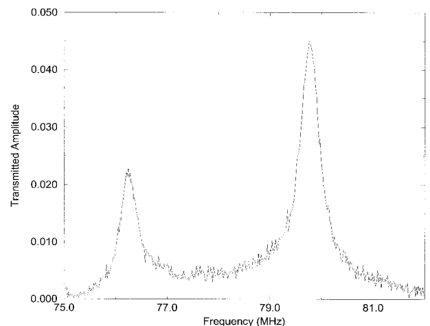
Fig. 4. Eigenfrequencies for the substrate inside the cavity. The sapphire substrate birefringence causes a splitting of the cavity TEM 01 resonance.
