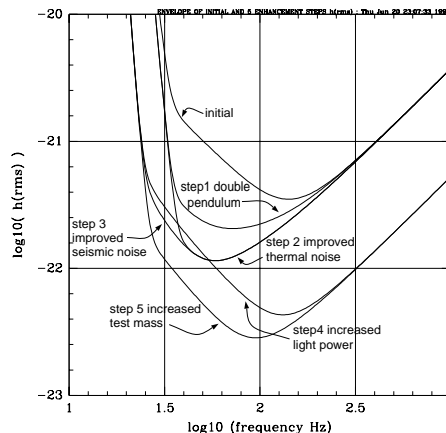
Figure 7: The improvements in h_{\text{rms}} \equiv h(f) \cdot \sqrt{f} associated with the steps outlined in the LIGO Advanced R&D proposal [9]. The logic of the steps is determined by the assumption that compact binary coalescences are the most likely source to be detected, hence the importance of improving the sensitivity near 100 Hz. The improvements associated with the double suspension, reduction in the thermal noise and increase in the test mass (steps 1, 2 and 5) are tightly coupled.
