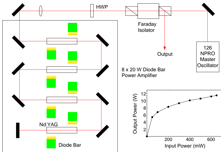
Figure 4: Design of the 10 W MOPA Nd:YAG laser being built by Lightwave Electronics, Inc. for the LIGO project. The master oscillator beam is double-passed through the amplifier (HWP is a half-wave plate).
