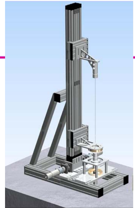
Fiber pulling fixture
