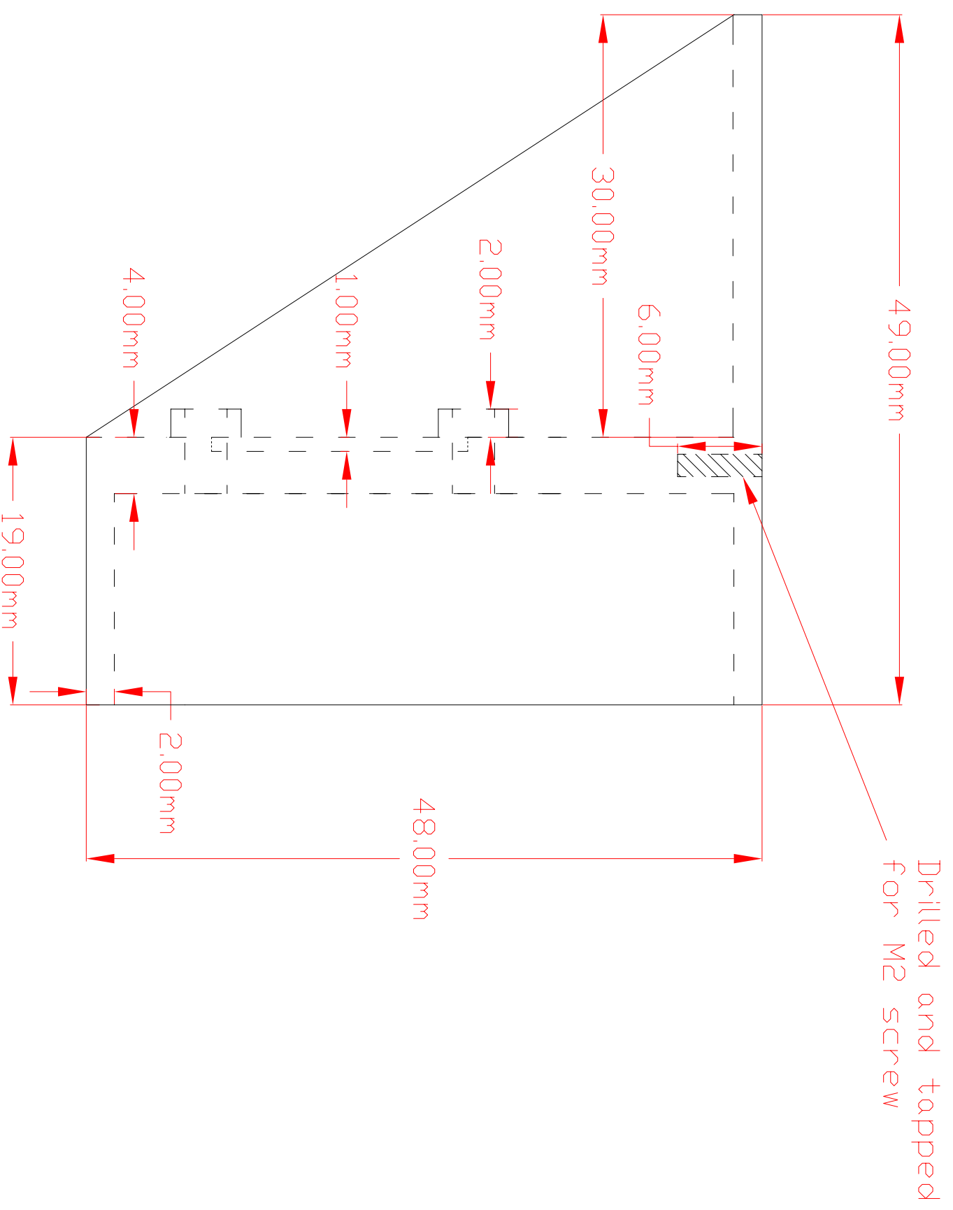
DCPD Heatsink - Left Side View
