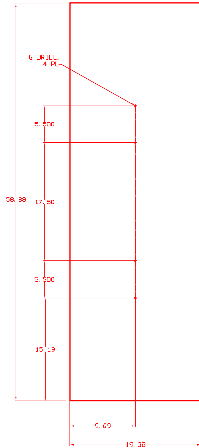
-2 20X59 LID MAT'L: 6061-T6 ALUMINUM; 5 REQ'D.
