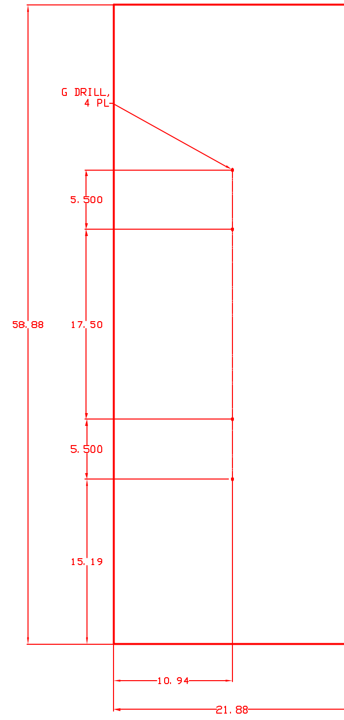
-3 22X59 LID MAT'L: 6061-T6 ALUMINUM; 2 REQ'D.
