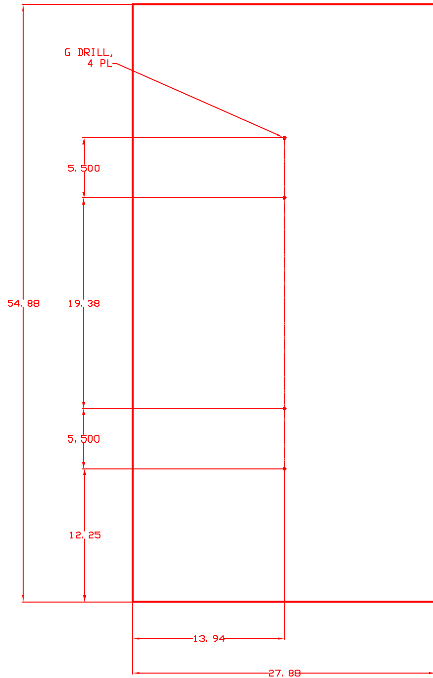
-1 28X55 LID MAT'L: 6061-T6 ALUMINUM; 1 REQ'D.
