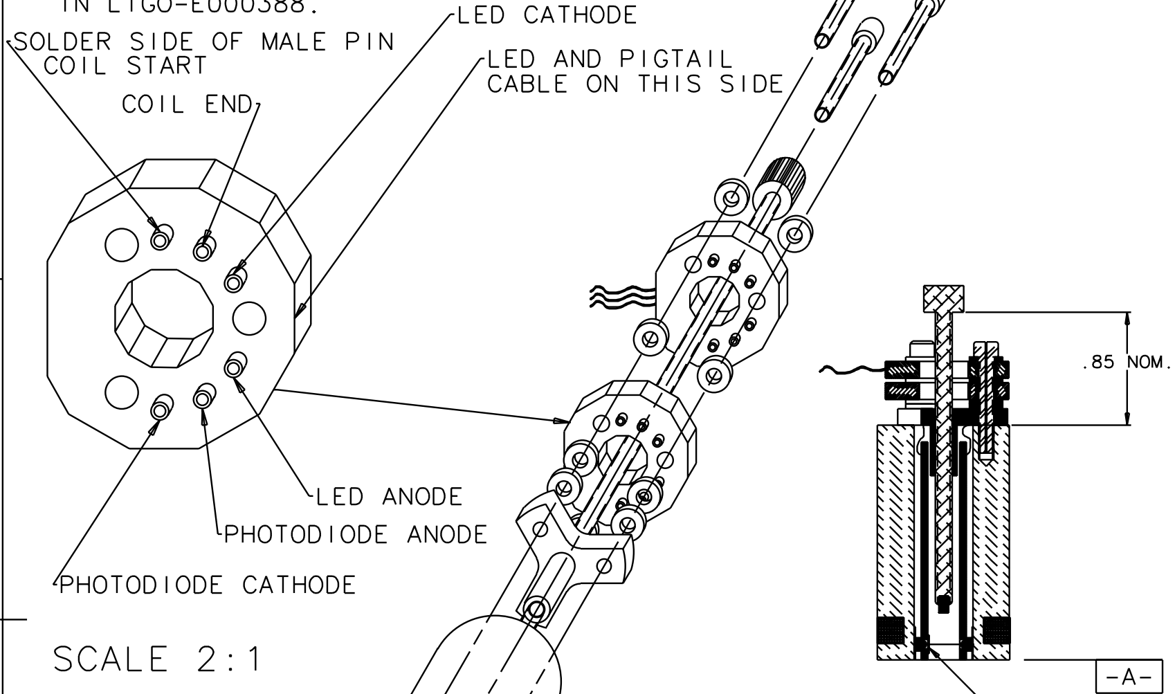
SECTION B-B (11) (6) A/R
