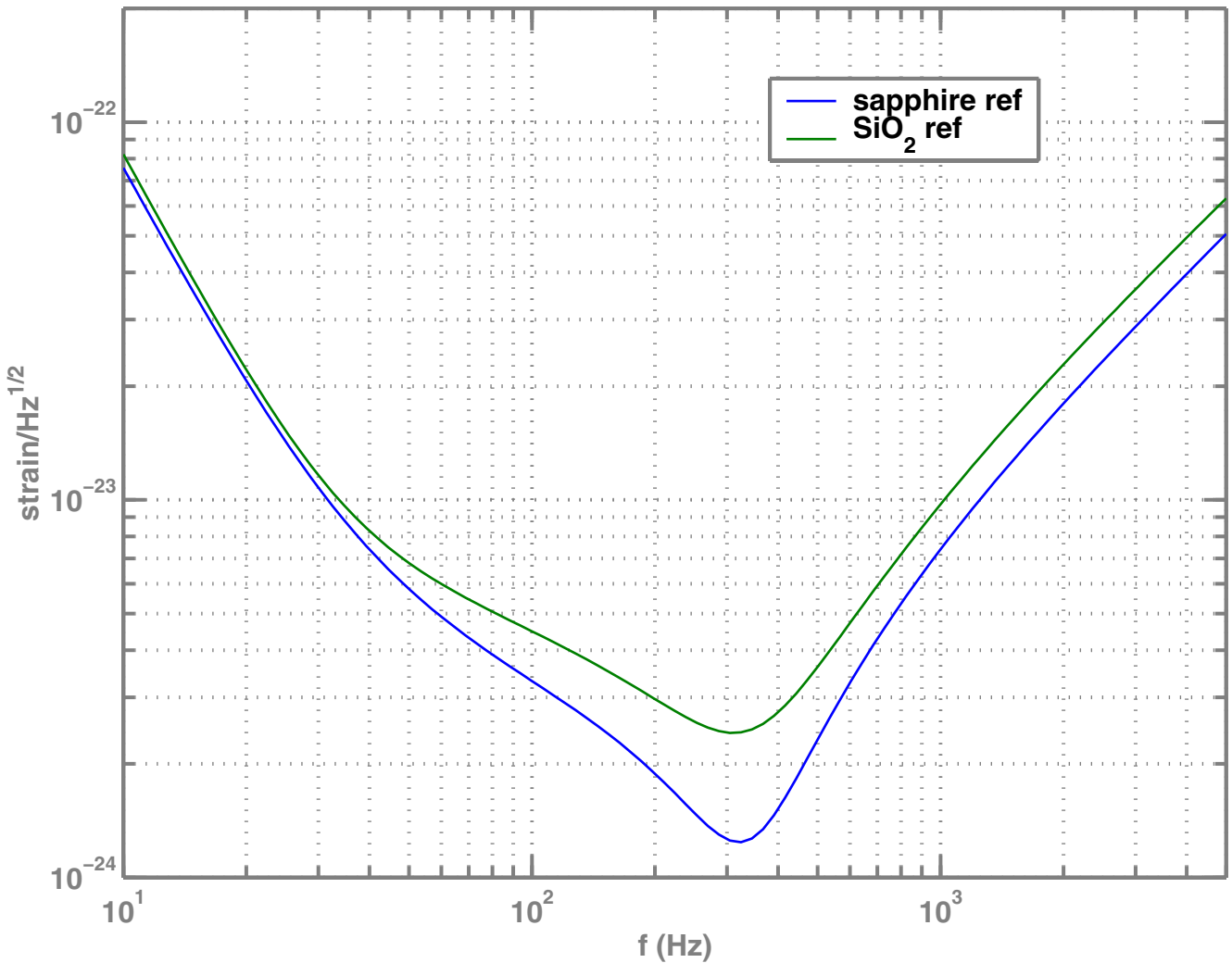
Comparison of sapphire and silica sensitivities
